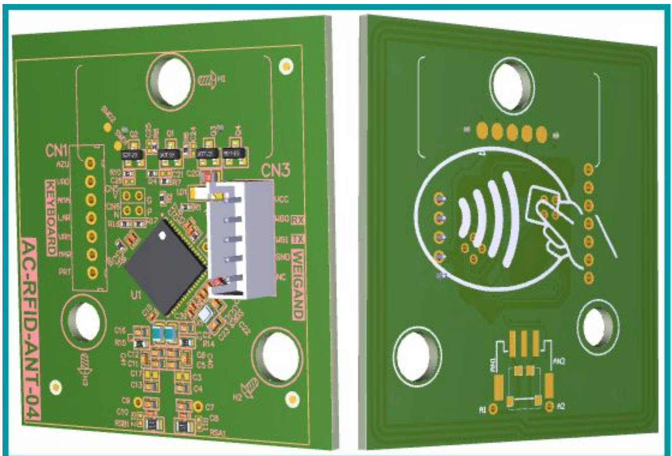
Subtitle: Front view of the board and rear view of the board.
